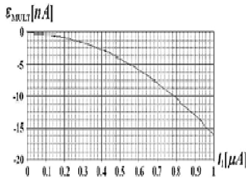
Fig. 4. Simulated linearity error for the multiplier/divider circuit.
