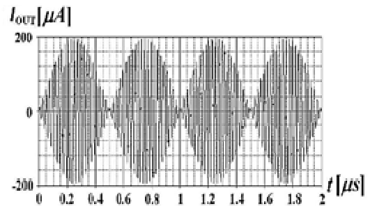
Fig. 5. I_{OUT} (I2) simulation for the multiplier/divider circuit.
