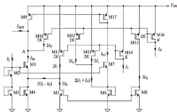
Fig. 2. Implementation of the multiplier/divider circuit.
