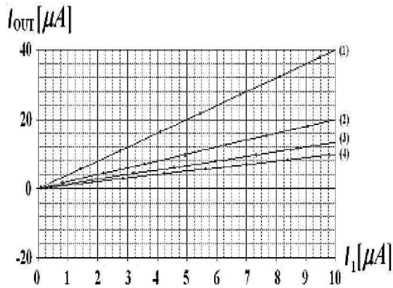
Fig. 3. I_{OUT} (I1) simulation for the multiplier/divider circuit
