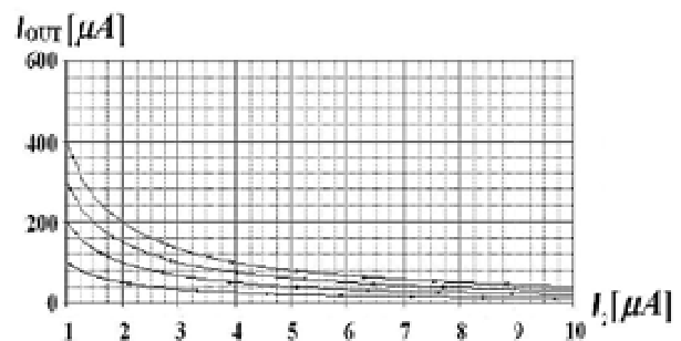
Fig. 6. I_{OUT} (t) simulation for the multiplier/divider circuit.
