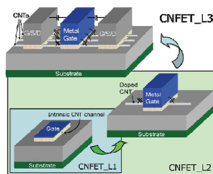
Figure 1. CNFET device structure with multiple nanotubes (CNFET_L3) and with a single tube (CNFET_L2) as illustrated in [2].
