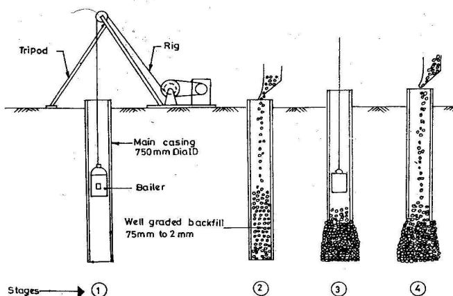
Fig. 2 Formation of Stone Column using Pre Bored Hole
