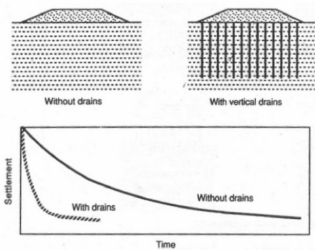
Fig. 1 Beneficial Effects of Vertical Drains (After Hausmann, 1990)
