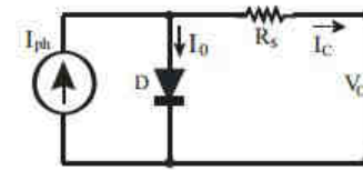
Fig.5 Simplified-equivalent circuit of photovoltaic cell
