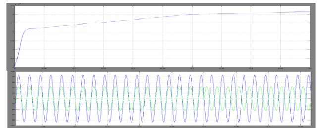
Fig.6.7 Upper: output power of the DFIG; Lower: AC side voltage versus current (Voltage times 1/3 for comparison).
