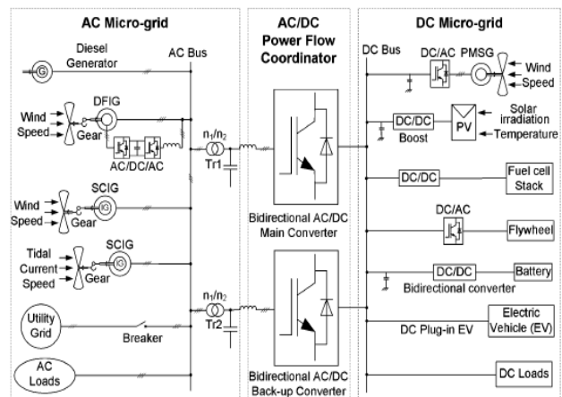
Fig.3 A hybrid ac/dc microgrid system
