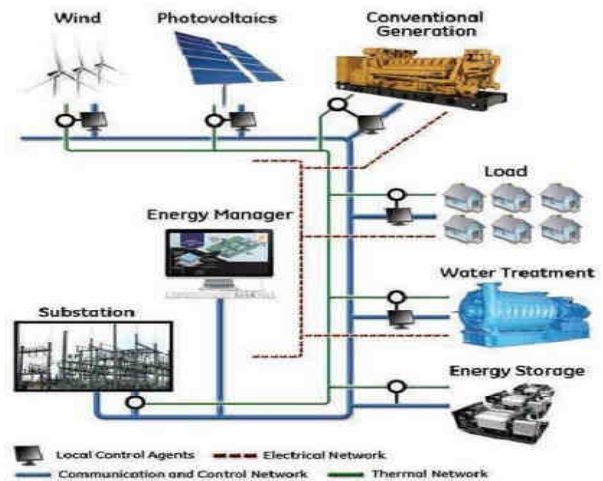
Fig.1 Micro-grid power system
