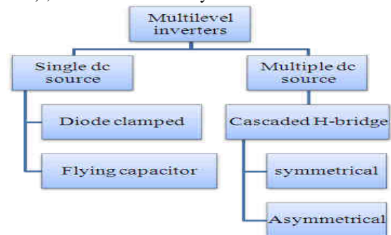
Fig.6 Classification of multilevel Inverters
