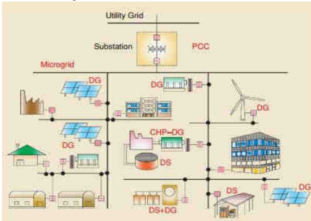
Fig.2 Microgrid structure including loads and DER units serviced by a distribution system
