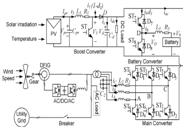
Fig.4 A compact representation of the proposed hybrid grid
