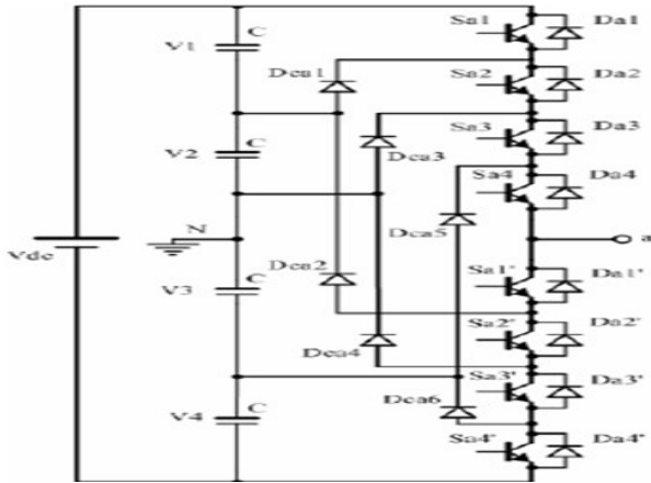
Fig.7 Five level diode clamped MLI
